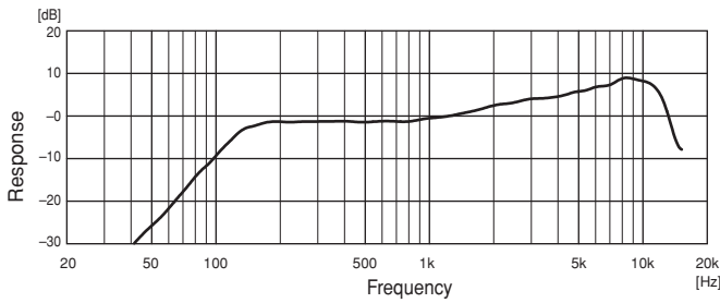
Frequency Response
